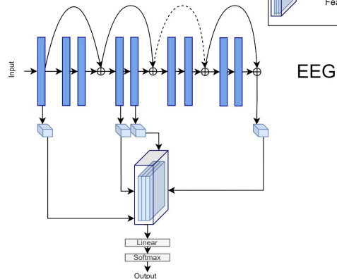
The BioDG baseline models
